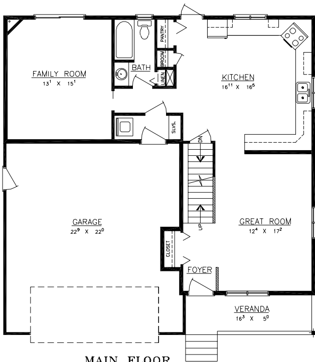
MAIN FLOOR AREA = 960 S.F.
